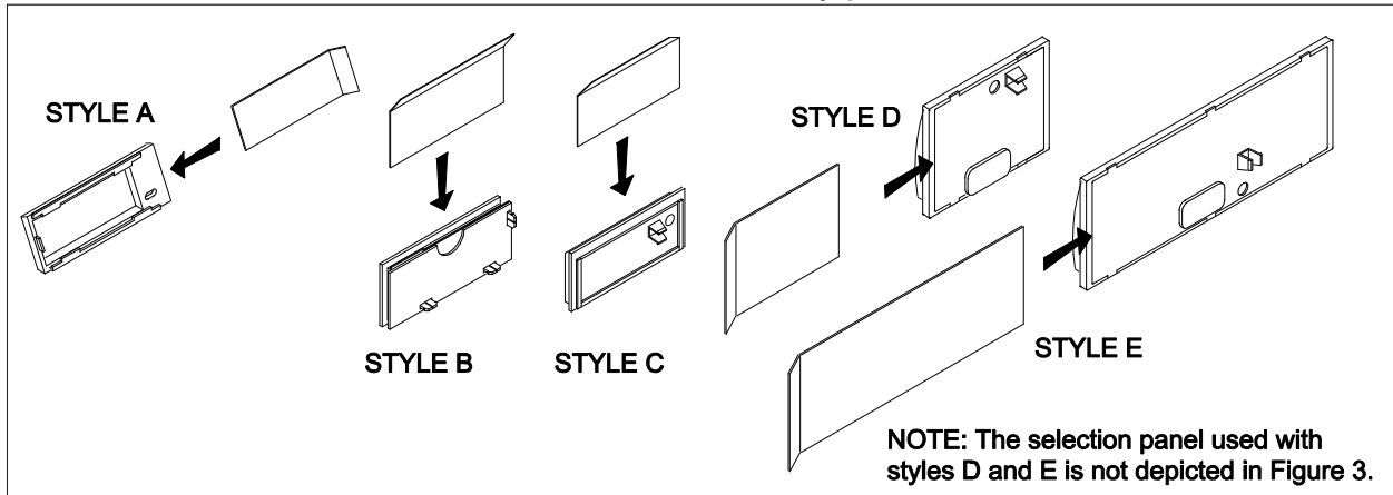
FIGURE 4 Part #1124016
